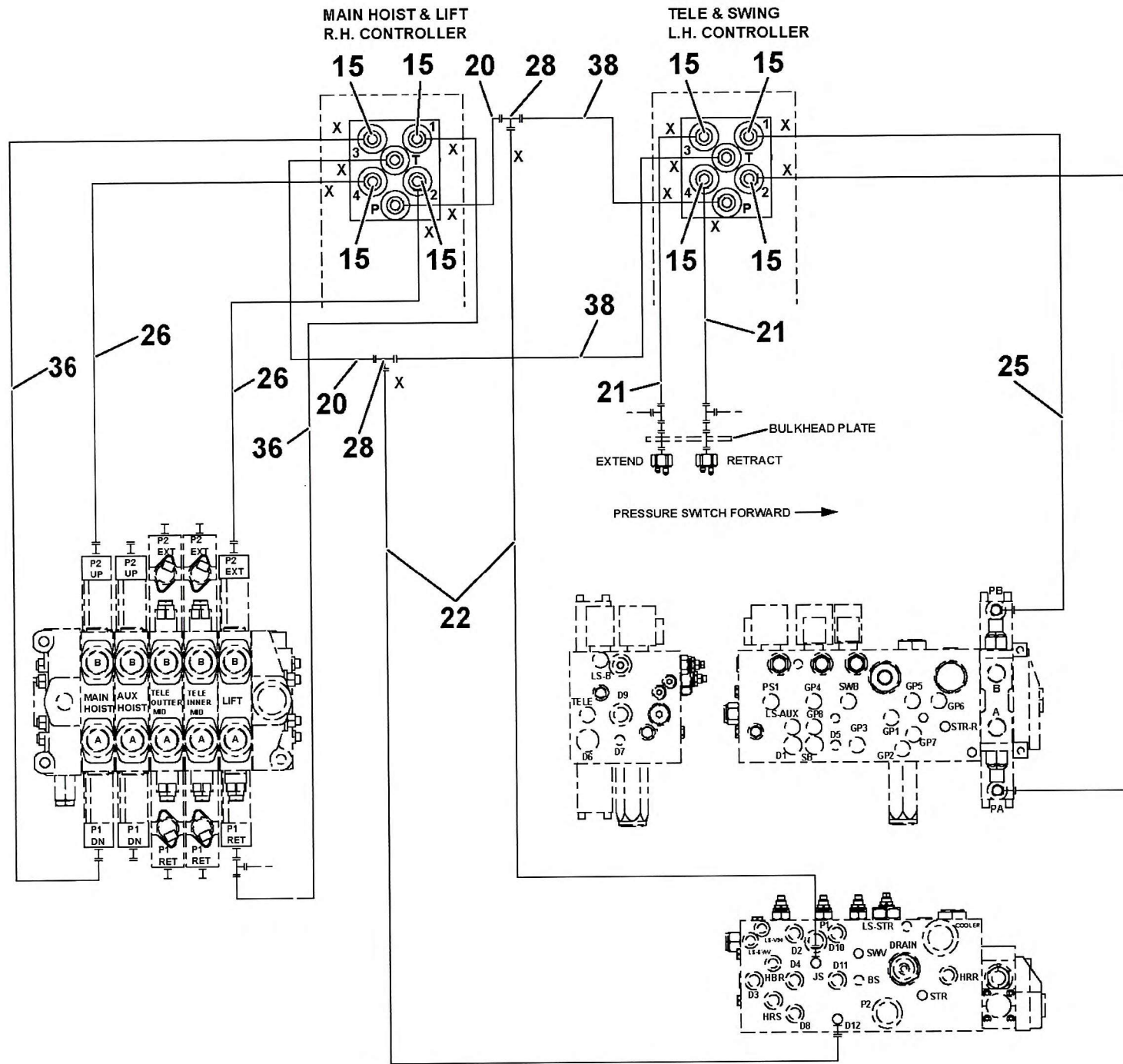
CONTROLLERS WITH FUTURE AUX HOIST
