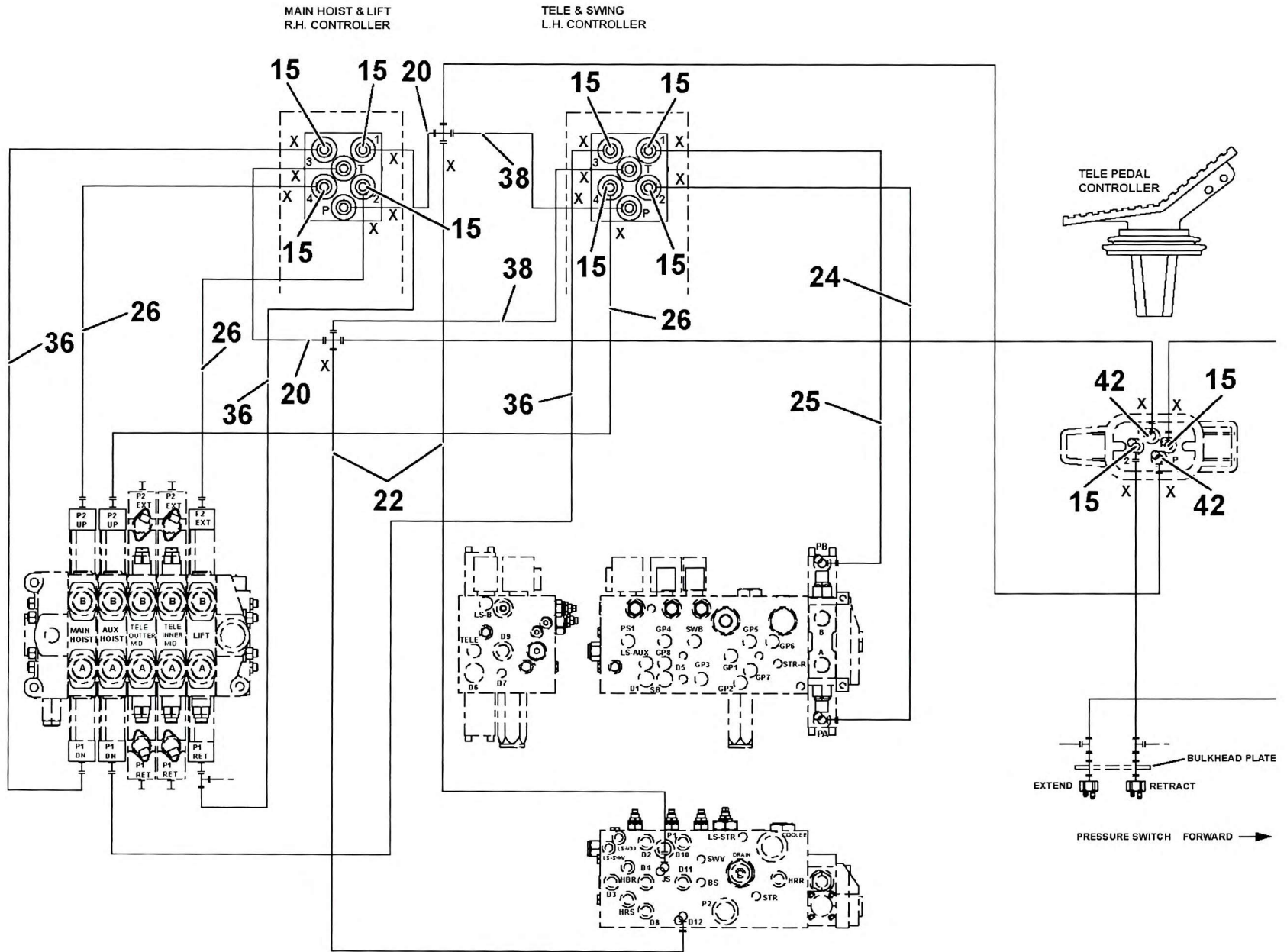
CONTROLLERS WITH MAIN AND AUX HOIST
