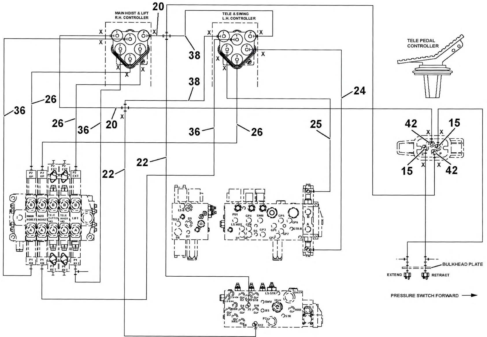
DUAL AXIS CONTROLLERS WITH MAIN AND AUX HOIST FOR CE CONFORMITY (OPTIONAL)
